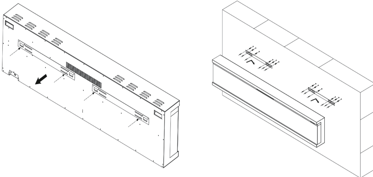
Illustration of wall bracket for model EF-443/72, EF-444/84
